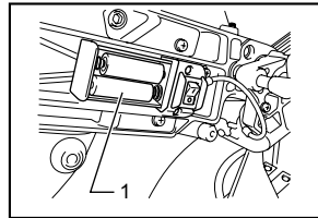
1. Dry cell
